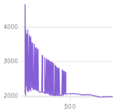
time/exclusive...ie/get_rollouts
