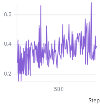
memory/mb_p...lpute_logprobs
