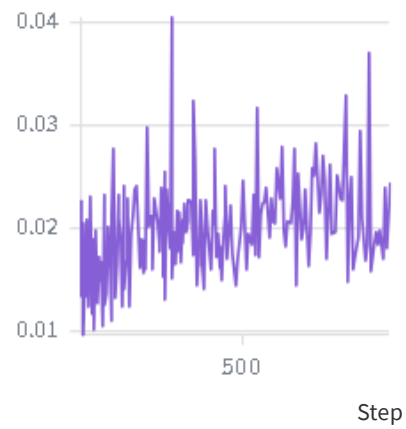
system_throughput_per_second
