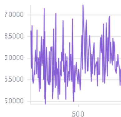
memory/mb_peak/odel_backward
