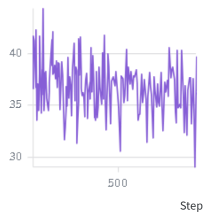
system_throughput_per_second
