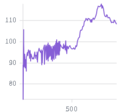
time/inclusive...pute_gradients
