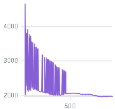
time/inclusive...ie/get_rollouts
