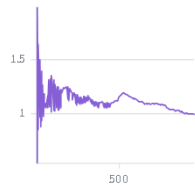
time/exclusive...gradient_steps
