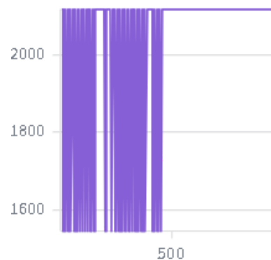
memory/mb_peak/setup_model
