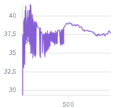
time/exclusive...ompute_probs
