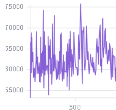
memory/mb_peak/pute_logprobs
