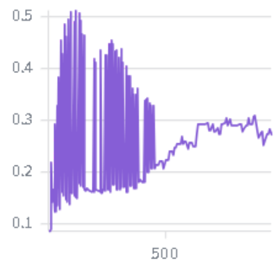
time/exclusive...optimizer_step
