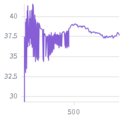
time/inclusive...ompute_probs
