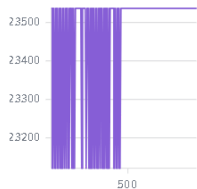
memory/mb_peak/tial_stress_loss
