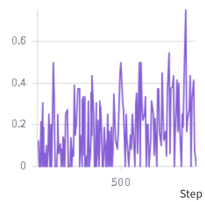
filtered_rollout...uccess_rate__2
