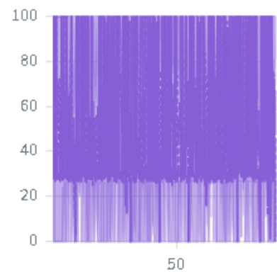
GPU Utilization (%)
