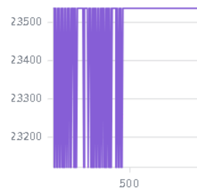
memory/mb_peak/stress_forward
